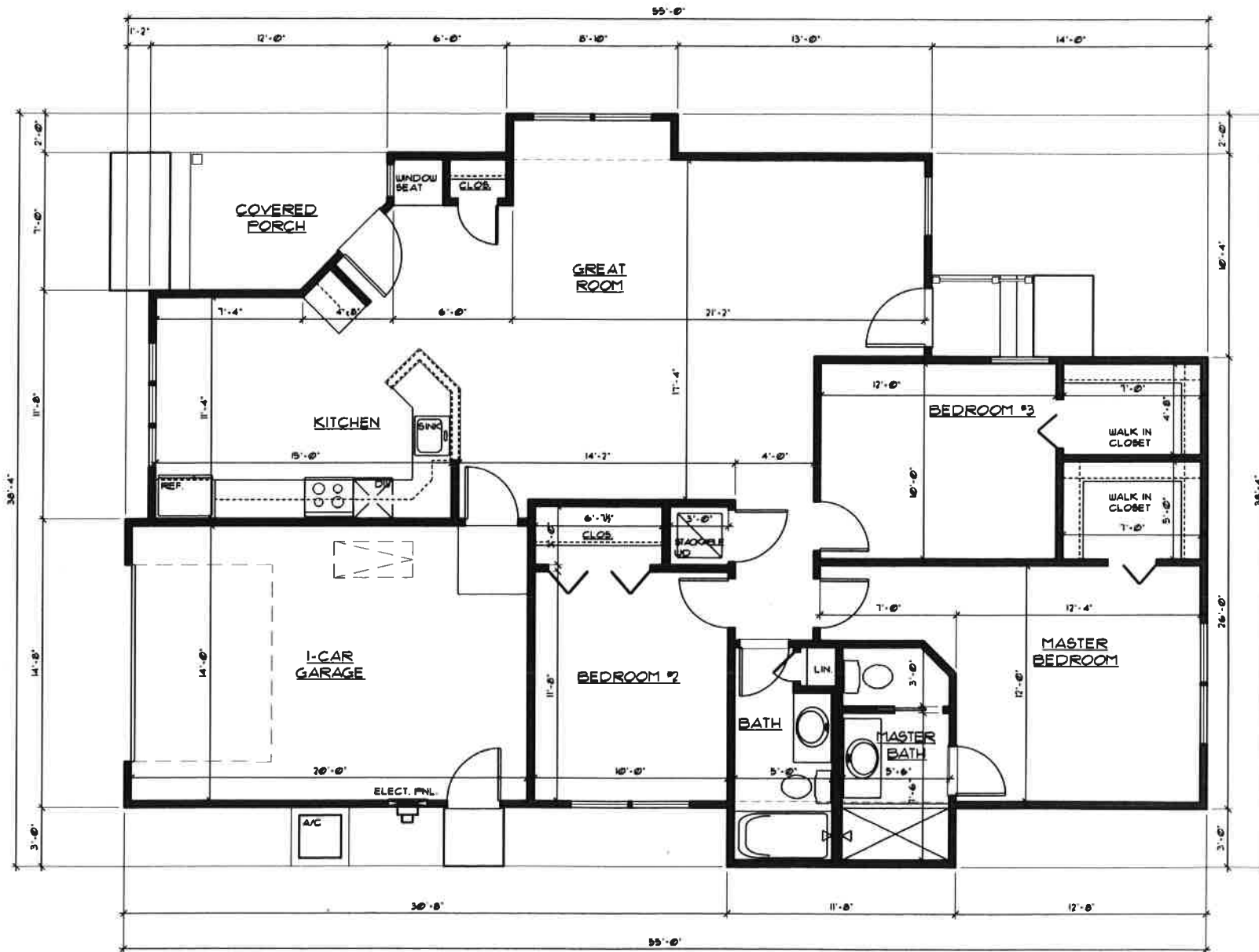
1ST FLOOR PLAN 1,343 SQ. FT. LIVING SPACE 303 SQ. FT. GARAGE SPACE
